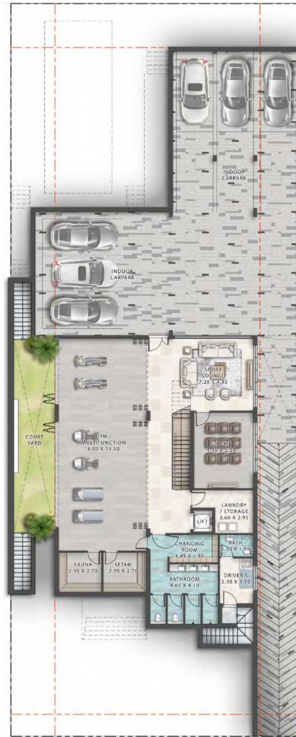
BASEMENT FLOOR
