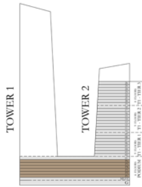
KEY SECTION-T2
