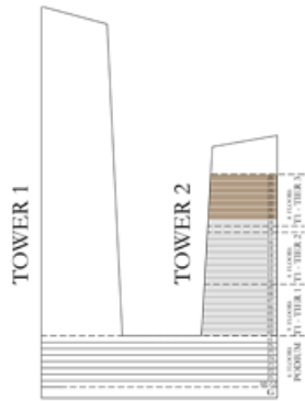
KEY SECTION-T3
