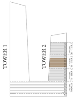
KEY SECTION-T2
