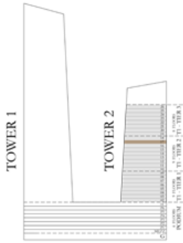
KEY SECTION-T2
