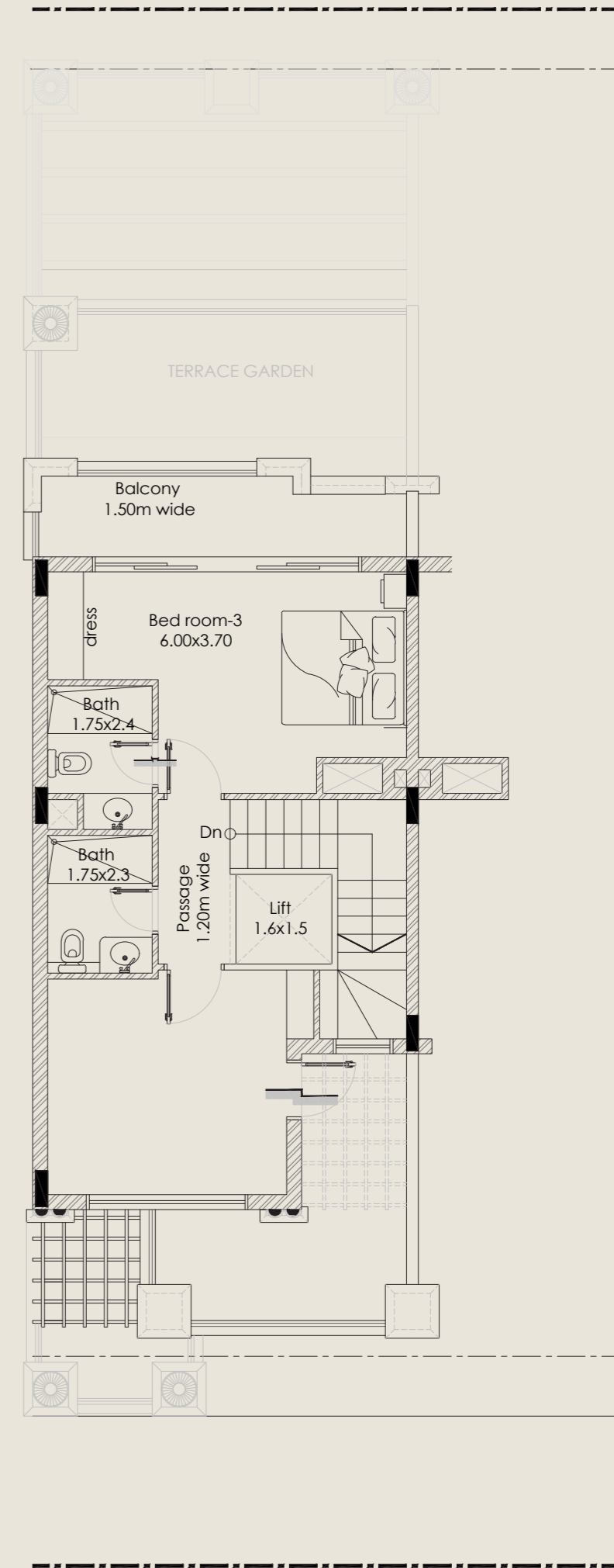
SECOND FLOOR
