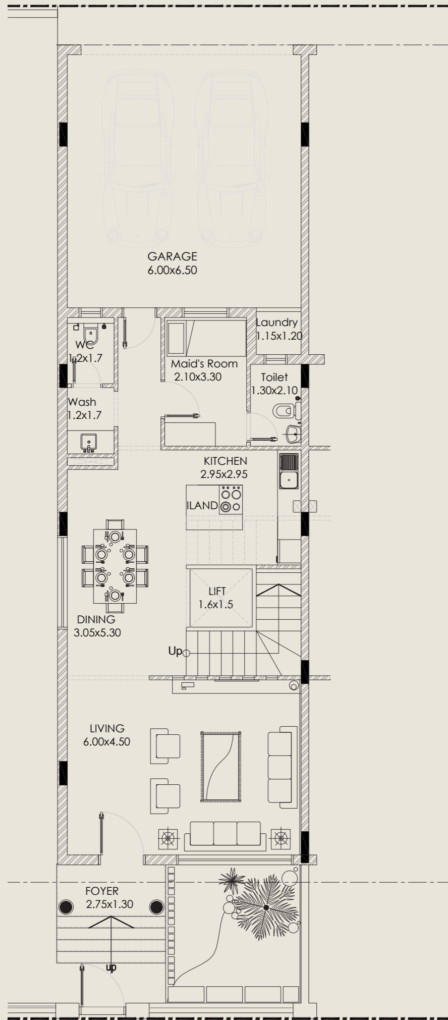
GROUND FLOOR
